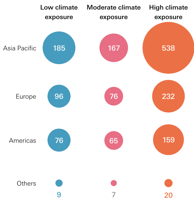
Region breakdown (2023/2024)
